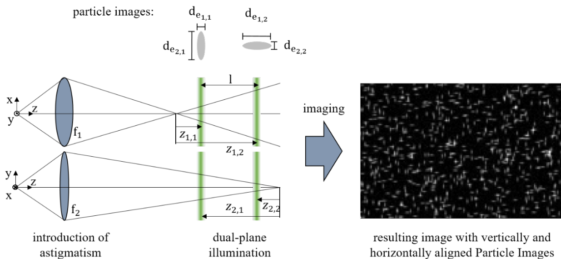
Figure 1: Optical system of a DPSA configuration (Kling et al. 2019). Illustration of the particle image dimensions in dependence of the focal lengths, the out-of-focus distances, the aperture and the optical magnifications. Exemplary image with horizontally and vertically aligned particle images.
