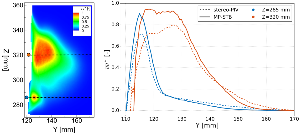
Figure 7: Left : wall-normal Reynolds stress component at X = 605 \text{ mm} obtained from ensemble averaging of the MP-STB results; black lines indicate the location of the profiles shown on the right. Right : wall-normal component of the Reynolds stresses at two span-wise locations ( Z = 285/320 \text{ mm} ); comparison between MP-STB and stereo-PIV results.
