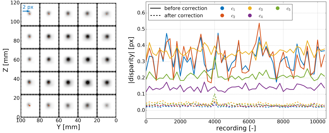
Figure 5: Left : result from the first iteration of single-image VSC for the complete five-camera imaging system making use of an actual recording during wind-tunnel operation; disparity map for camera c_2 . Right : time-history of the disparity before and after single-image VSC correction of the complete imaging system.
