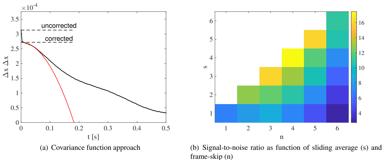
Figure 3: Improvement of the signal-to-noise ratio for a time signal at radial position r/R \approx 0.9 .
