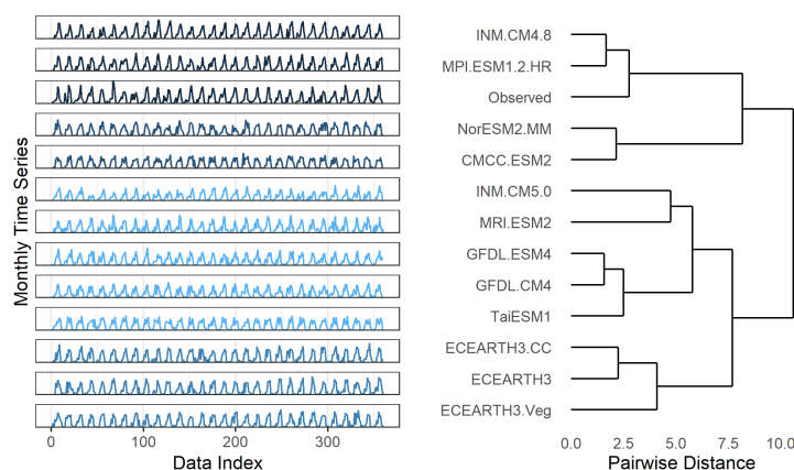
Figure 3. Clusters for the monthly precipitation series for the observed and climate model series (the left figure shows the cluster separation with blue color contrast, and the right figure shows the clustering of climate models and observed data in terms of time series similarities based on seasonal patterns).
