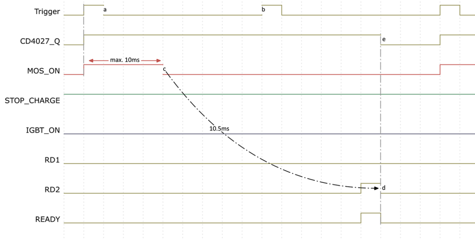
Fig. 11 Timing diagram of the control unit in case of irregular operation
